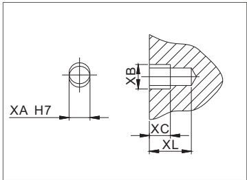
Detailed drawing of XX Part (XX部详细图)
